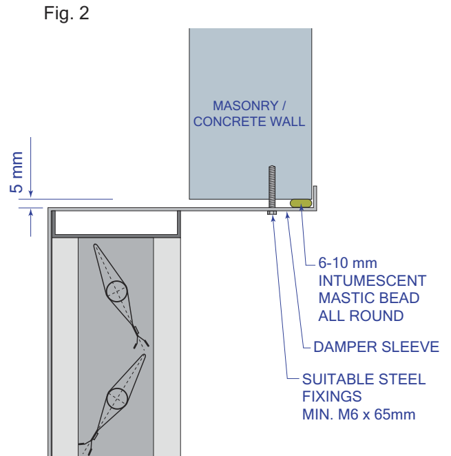
Sectional View
